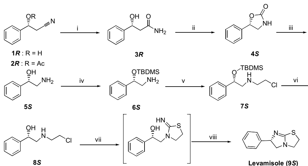
Scheme 2. Reagents and conditions: (i) H 2 O 2 , aq NH 3 ; (ii) Pb(OAc) 4 , pyridine; (iii) NaOH, EtOH–H 2 O, reflux; (iv) TBDMS–Cl, imidazole; (v) 1,2-dichloroethane, K 2 CO 3 , 18-crown-6; (vi) TBAF, THF; (vii) KSCN, EtOH–H 2 O; (viii) SOCl 2 , CH 2 Cl 2 .
